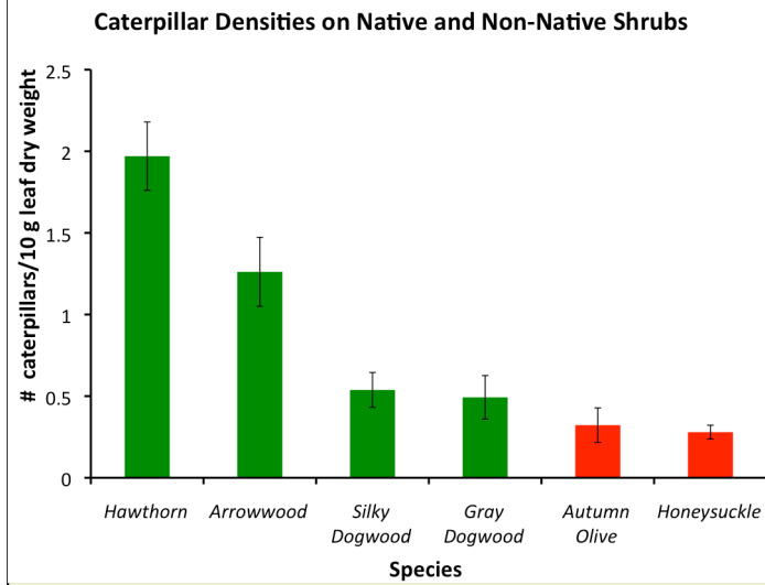
Figure 2. Research conducted in Pennsylvania state parks demonstrates that native shrubs host more caterpillars than exotic shrubs. In the chart below, green bars represent native species and red bars are exotic species. Each bar indicates the average number of caterpillars found per unit of leaf dry weight (S. Moon, Indiana University of PA).
